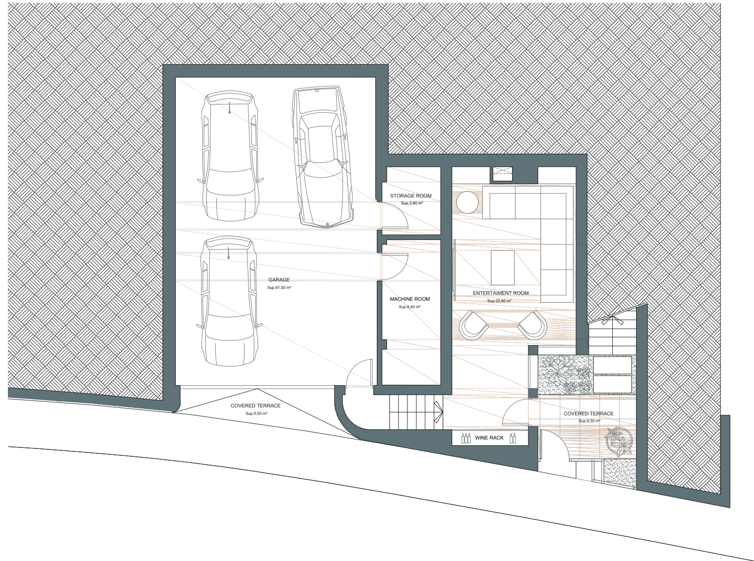
Basement
