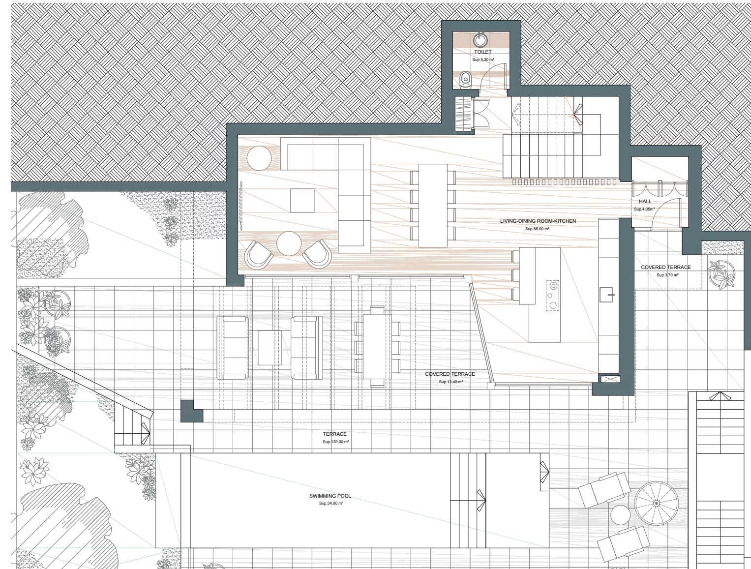
Ground floor
