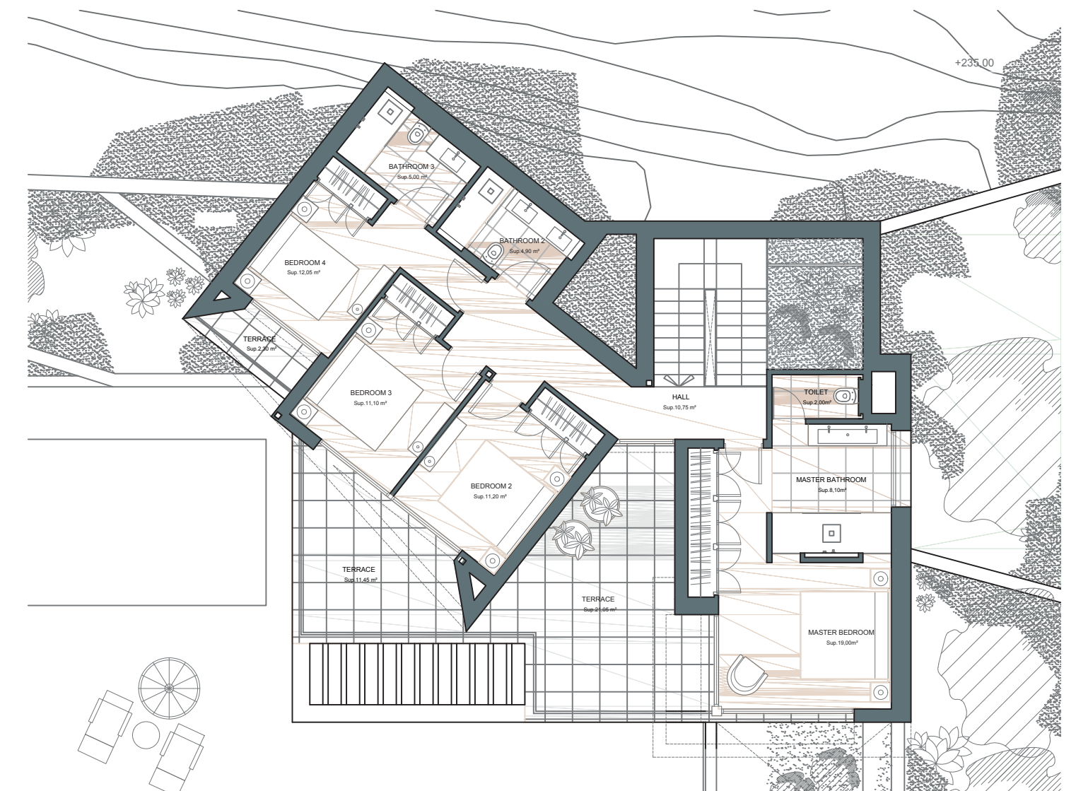
First floor
