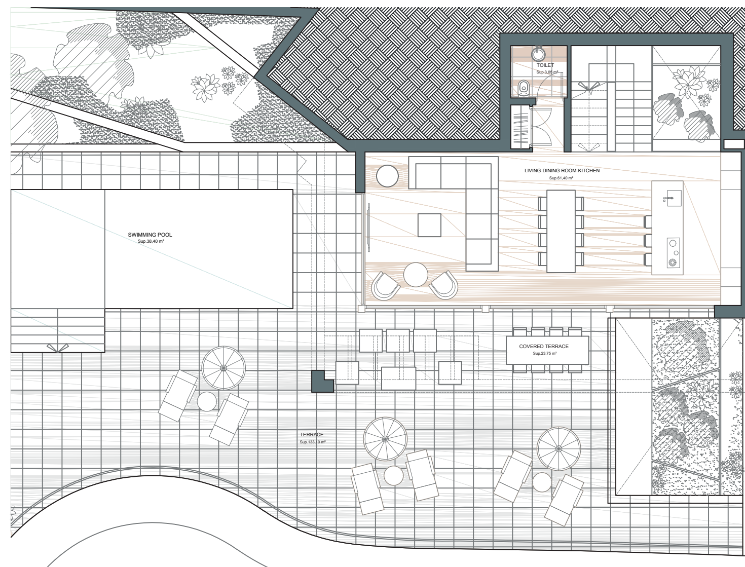
Ground floor
