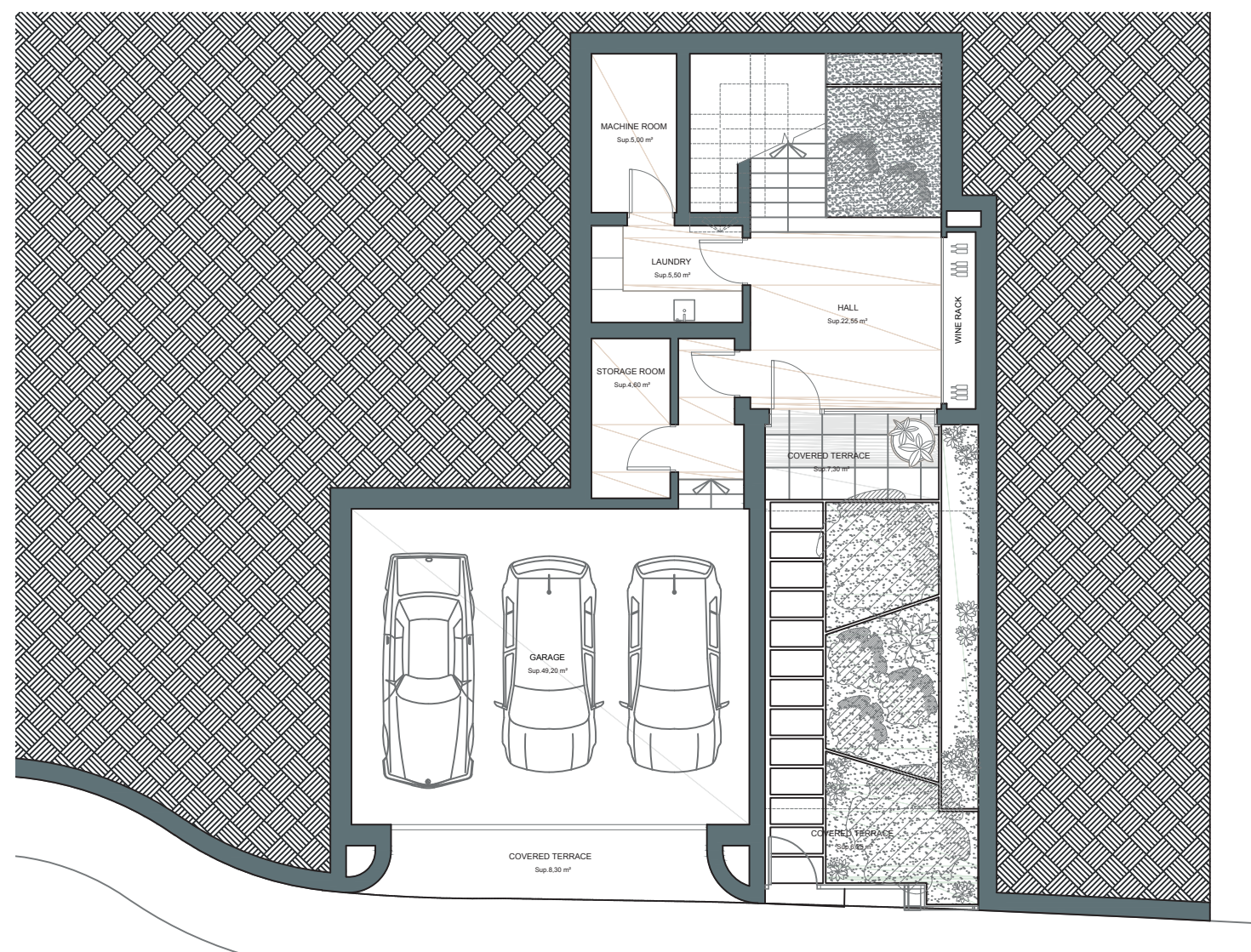
Basement
